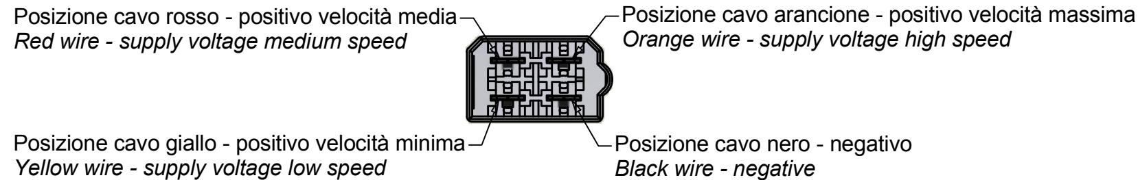
Vista frontale connettore tipo AMP Faston 180908-0 Front view AMP type 180908-0 connector
