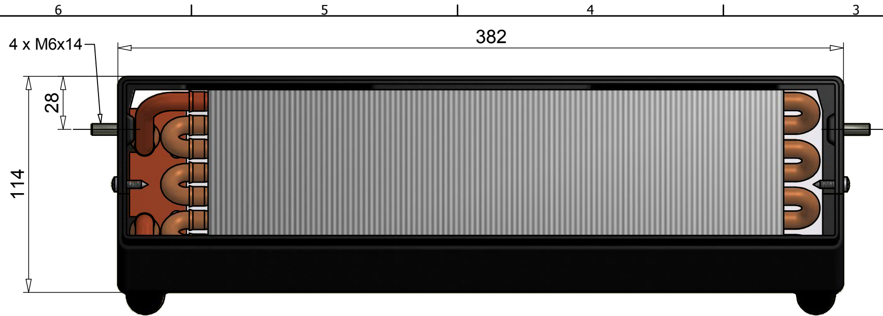
Collegamenti IN-OUT per tubi flessibili Ø16mm IN-OUT connections for Ø16mm flexible hoses
